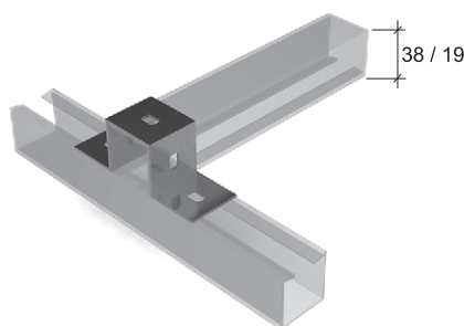
CANTONEIRA "ZZ"
