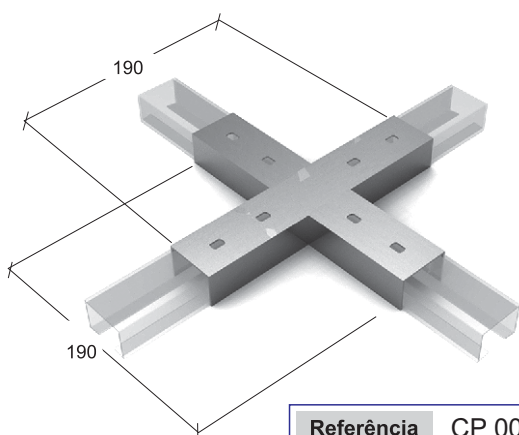
EMENDA "X"
