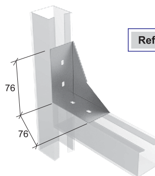
CANTONEIRA "L" 3 FUROS
