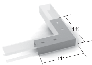
EMENDA "L"
