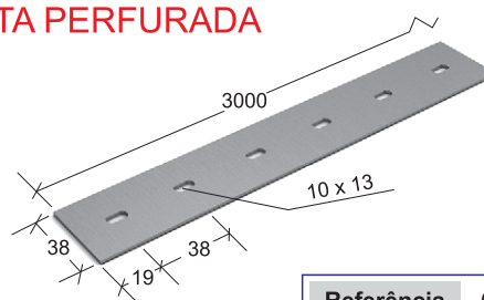
FITA PERFURADA
