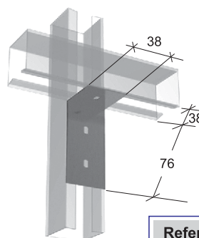
CANTONEIRA "L" 3 FUROS
