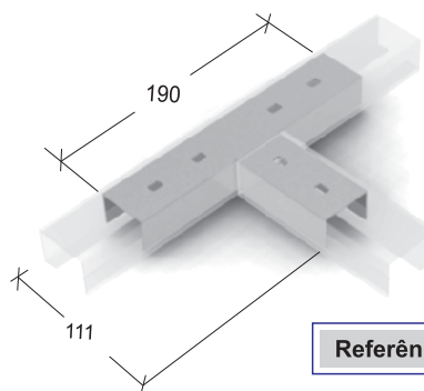
EMENDA "T"
