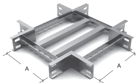
CRUZETA RETA
